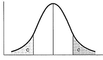
FIGURE A.2 AREA BEYOND Z
