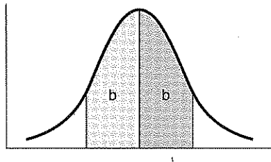
FIGURE A.1 AREA BETWEEN MEAN AND Z
